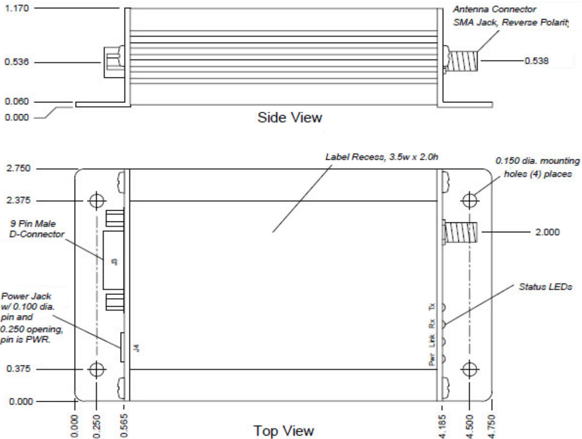
Figure 7: Mechanical Drawing
