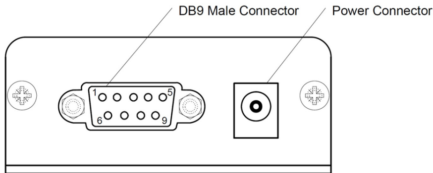
Figure 2: CL024-RS232
